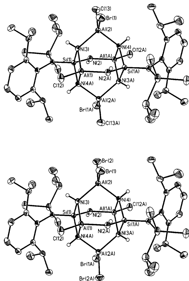
Figure 4. Crystal structures of 6a (top) and 6b (bottom) (hydrogen atoms are omitted for clarity). Selected bond lengths [pm] and angles [°] for 6a : Al(2)–Br(1) 232.27(9), Al(2)–C(13) 197.1(13), C(13)–Al(2)–Br(1) 110.0(5); 6b : Al(2)–Br(2) 220.6(5), Br(2)–Al(2)–Br(1) 113.4(2)
